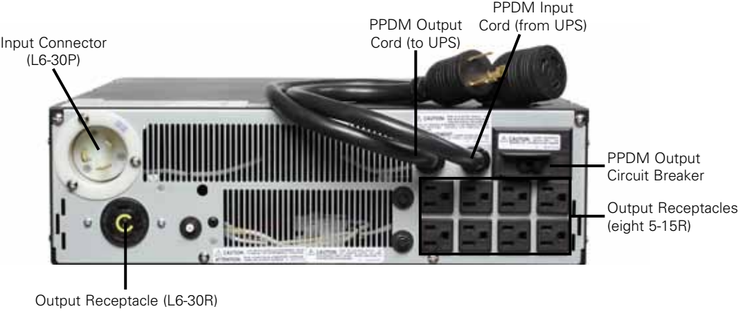
PPDM back panel input and output configuration
